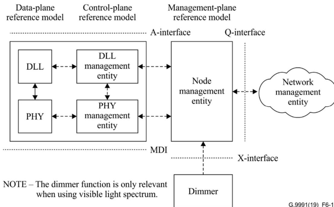
Figure 32: Management model of G.9991
