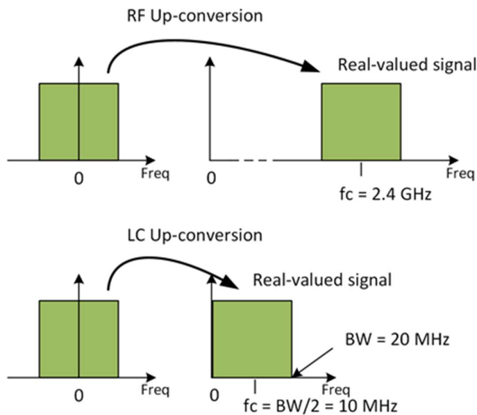
Figure 20: Reuse of existing signal processing schemes from RF for LiFi
