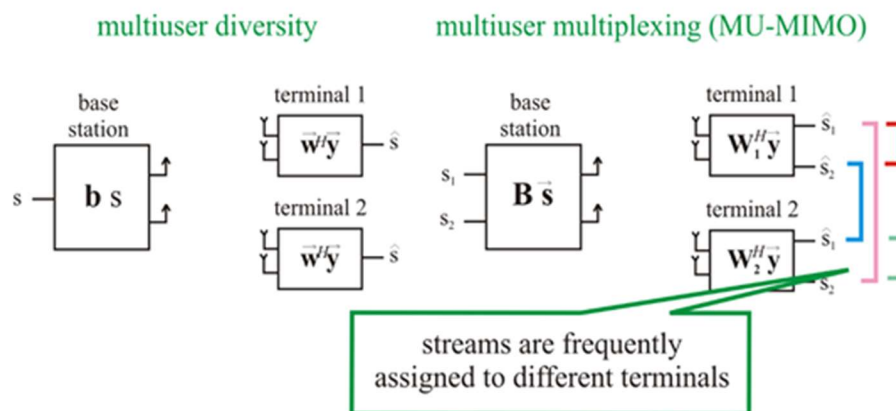
Figure 23: Multiuser diversity vs. multiuser multiplexing
