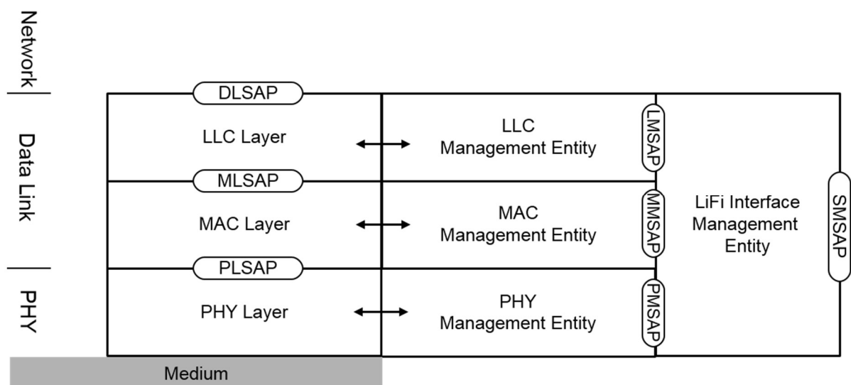
Figure 13: Basic reference architecture
