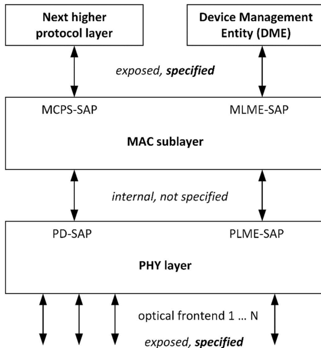
Figure 29: IEEE P802.15.13 reference architecture
