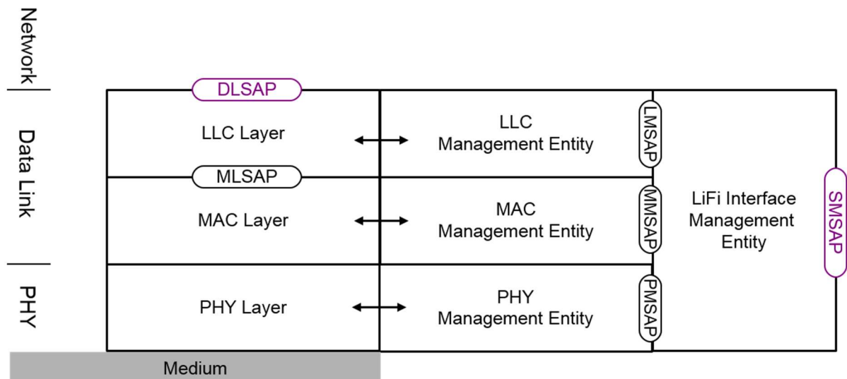
Figure 15: Open interfaces in reference architecture model
