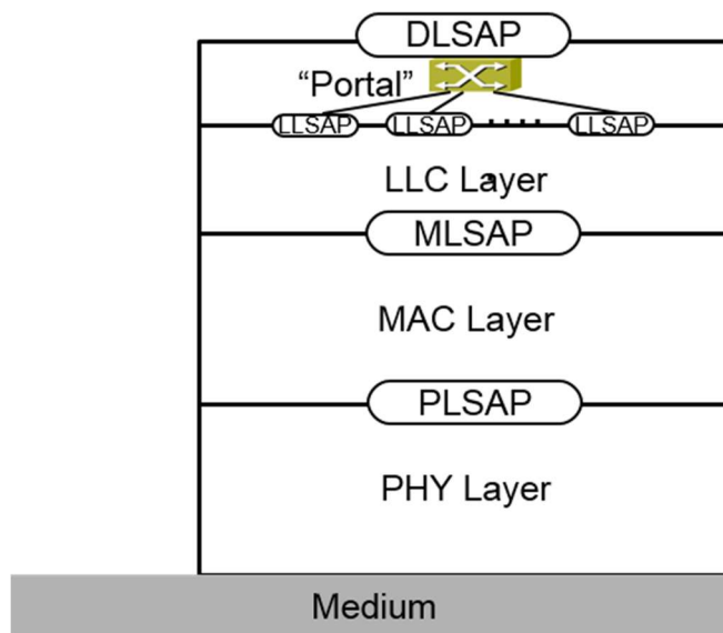
Figure 17: Link layer extensions for AP functionality
