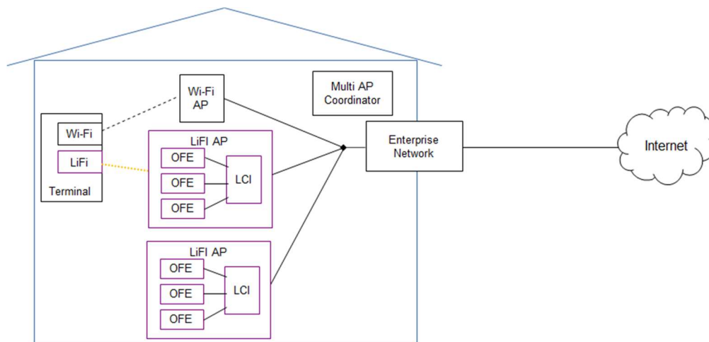
Figure 1: Office – system architecture overview
