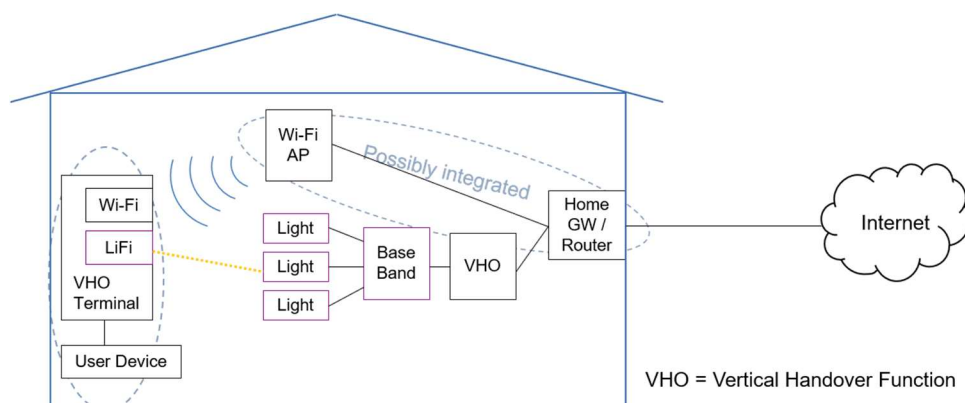
Figure 7: System architecture overview of consumer home use case
