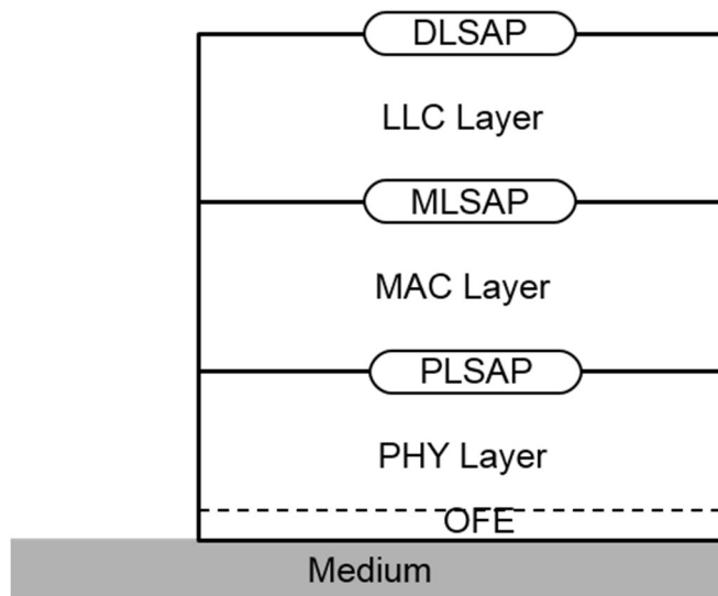
Figure 18: Signal conversion into medium
