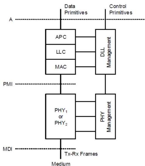
Figure 31: Open interfaces of G.9991
