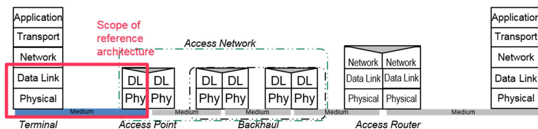
Figure 11: Scope of reference architecture in end-to-end communication architecture
