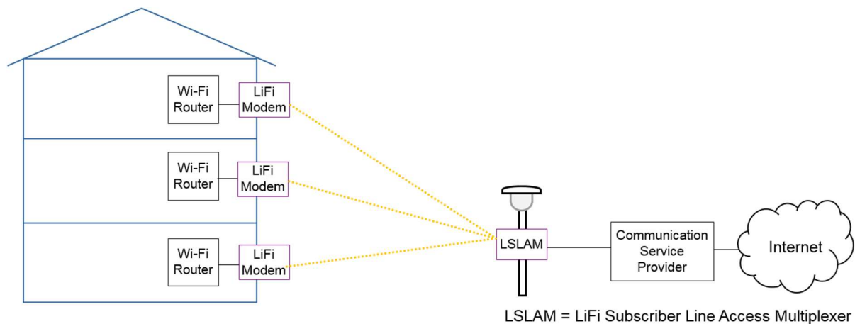
Figure 10: System architecture of FWA use case
