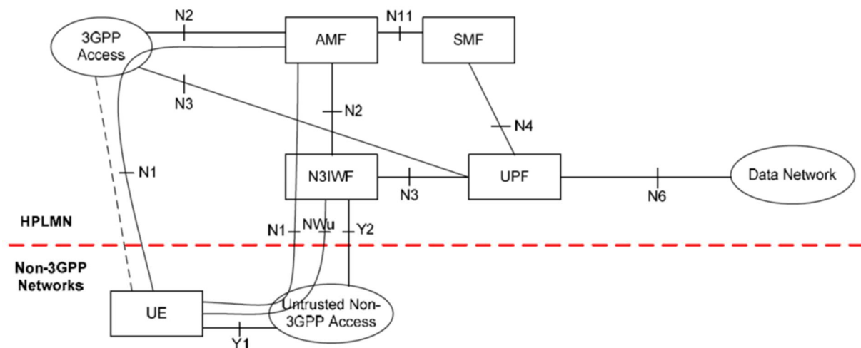
Figure 34: TS 23.501 reference architecture for integration of non-3GPP access technologies
