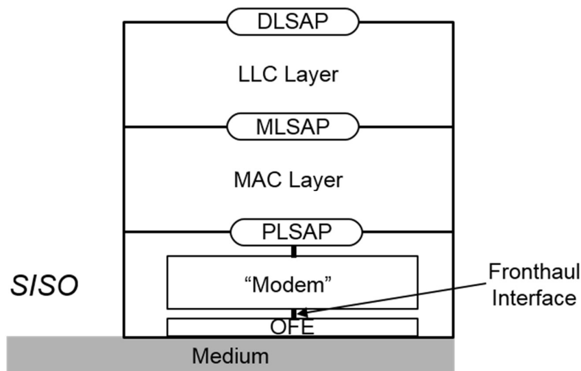
Figure 19: Representation of fronthaul in reference model
