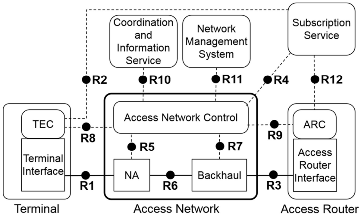
Figure 33: IEEE 802.1CF network reference model
