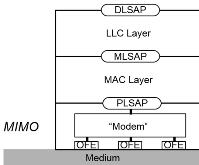
Figure 24: MIMO extension to reference model
