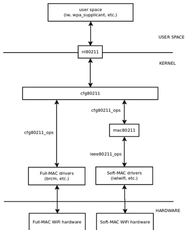
Figure 28: Implementation of IEEE 802.11 within mac80211
