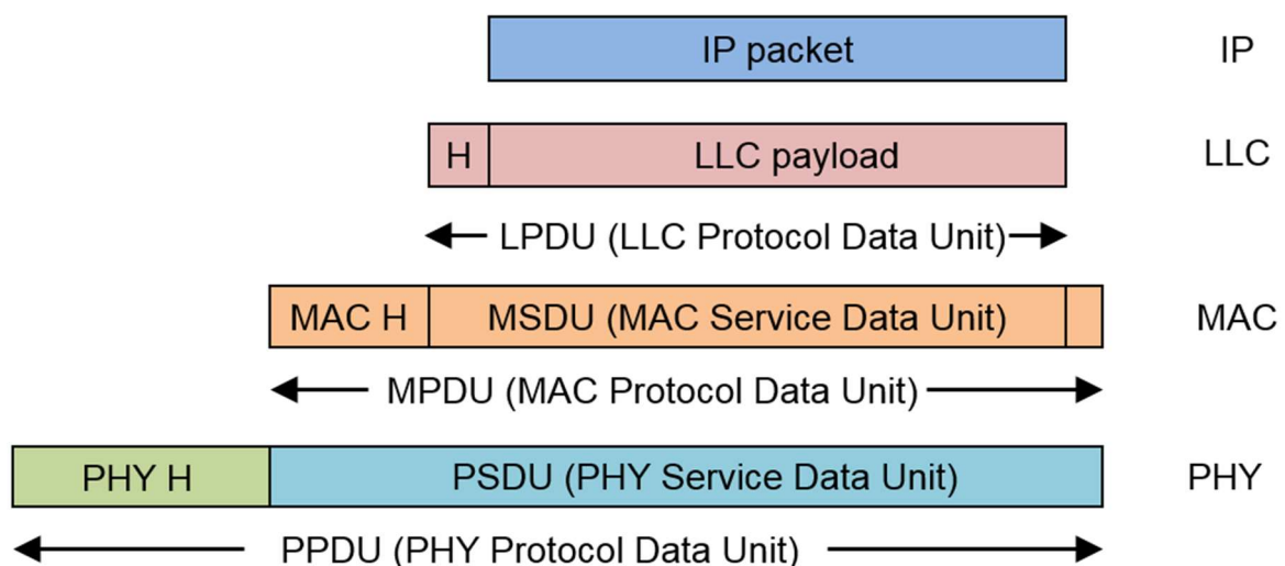
Figure 14: Protocol data unit concatenation through successive preceding of header information
