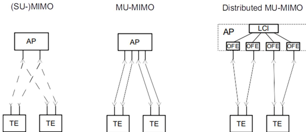
Figure 22: Different configurations when using multiple antennas/OFEs for single and multiple users
