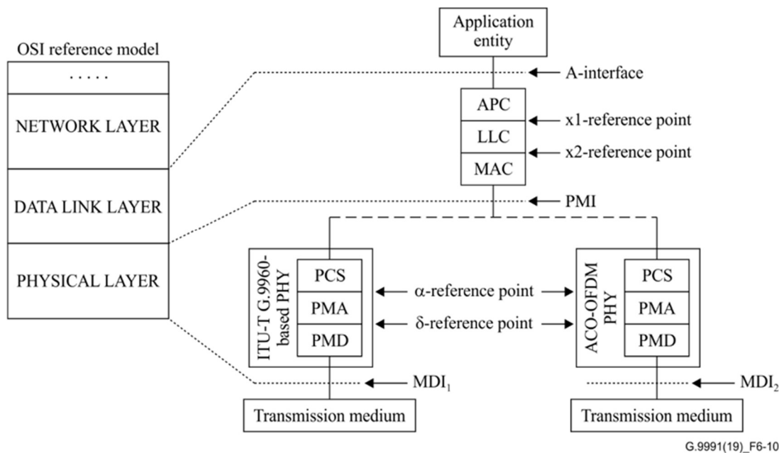
Figure 30: Datapath reference architecture of G.9991
