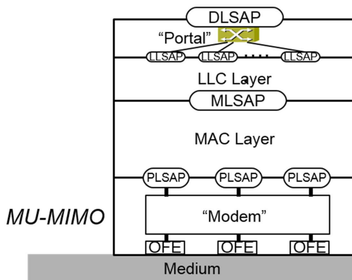
Figure 26: Comprehensive LiFi reference model of data path
