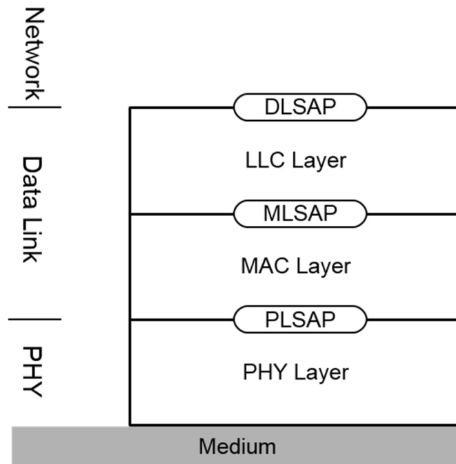
Figure 16: Datapath section of basic open reference architecture
